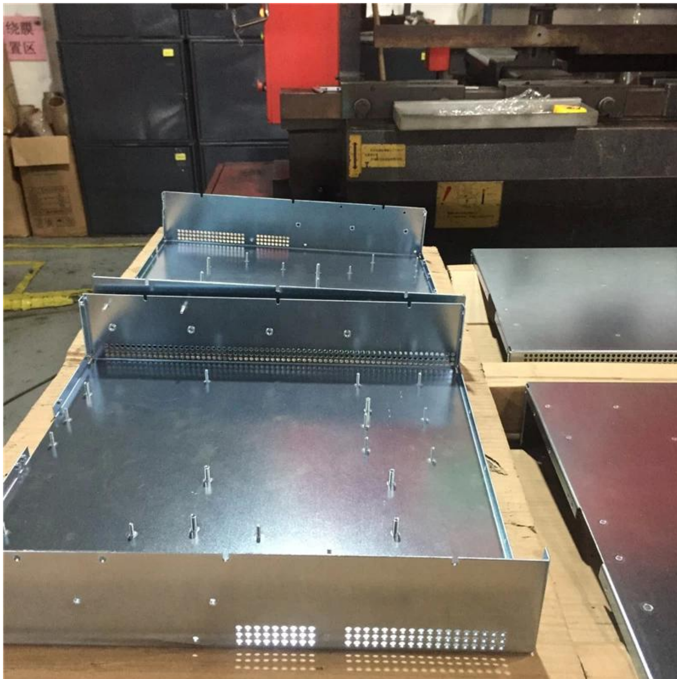
Manufacturing process
